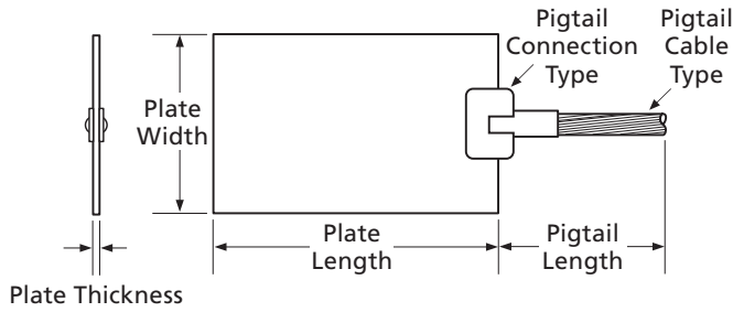
Terminated Pigtails
